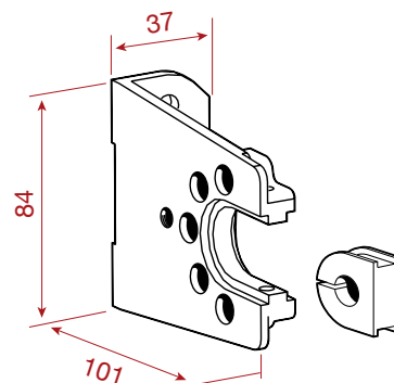
Mounting Bracket Face or Top Fix (mm)
