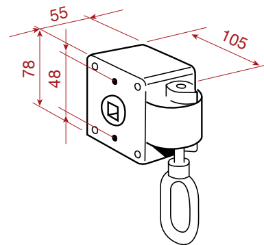
Gearbox 13.1 (mm)
