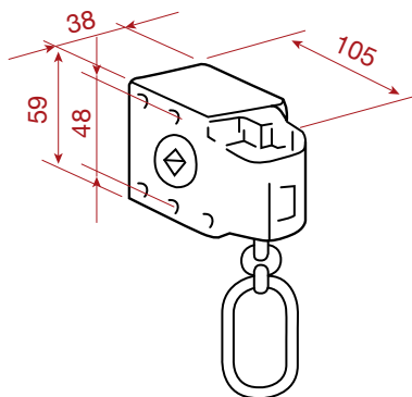
Gearbox 7:1 (mm)
