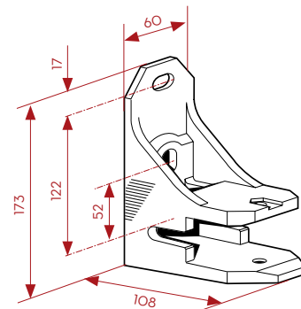
Fetuna Facefix Bracket (mm)
