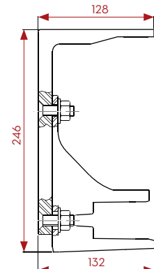
Fetuna Soffit Bracket (mm)
