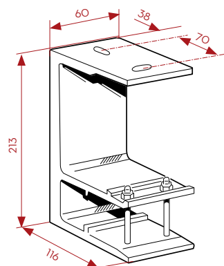
Horizon Soffit Bracket (mm)
